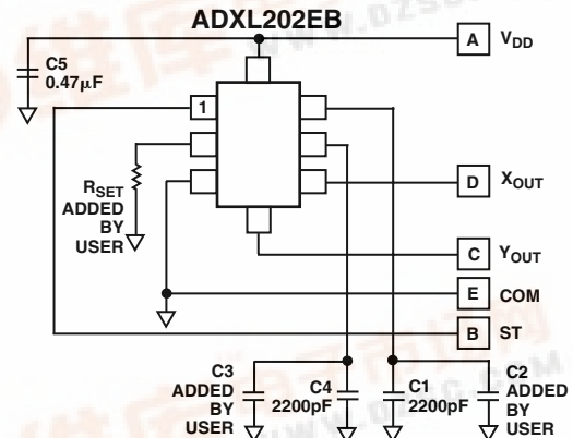
Figure 1. ADXL202EB Schematic
