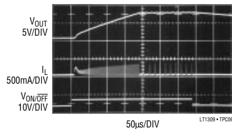
Start-Up Waveforms, I LOAD = 10mA
