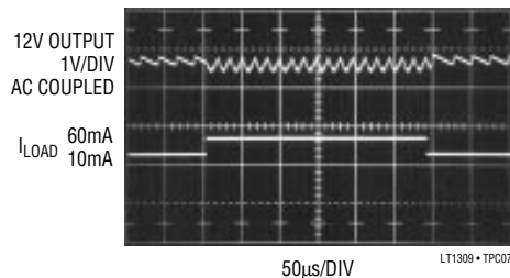
Load Transient Response, C OUT = 1µF
