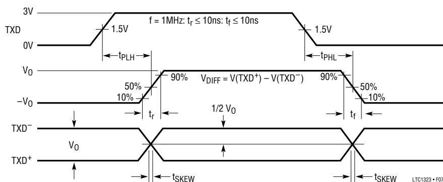
Figure 7. Differential Driver
