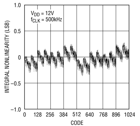
Integral Nonlinearity
