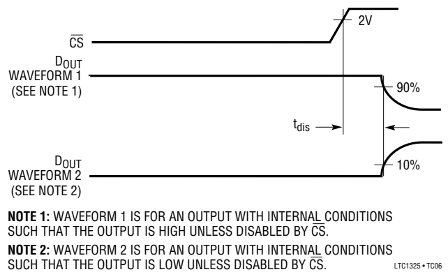
Voltage Waveforms for t_{dis}
