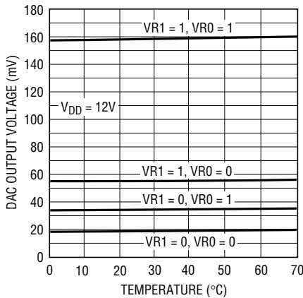
DAC Output Voltage vs Temperature
