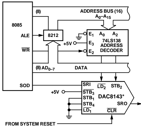
Figure 22. DAC8143—8085 Interface
