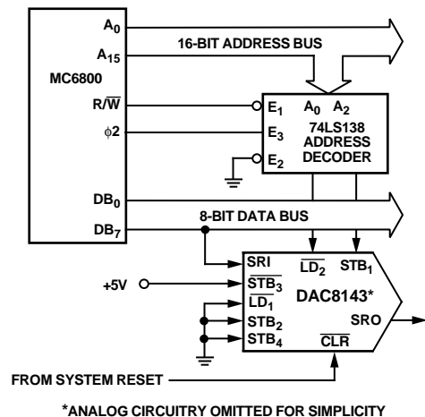
Figure 21. DAC8143—MC6800 Interface
