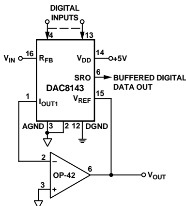
Figure 20. Analog/Digital Divider
