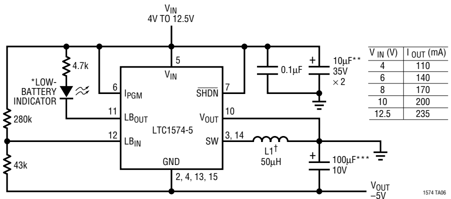
Positive to -5V Converter
