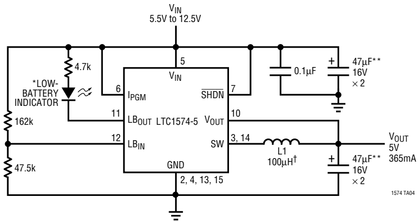
Low Dropout 5V Step-Down Regulator with Low-Battery Detection
