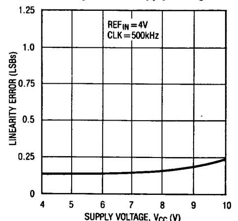
Linearity Error vs Supply Voltage
