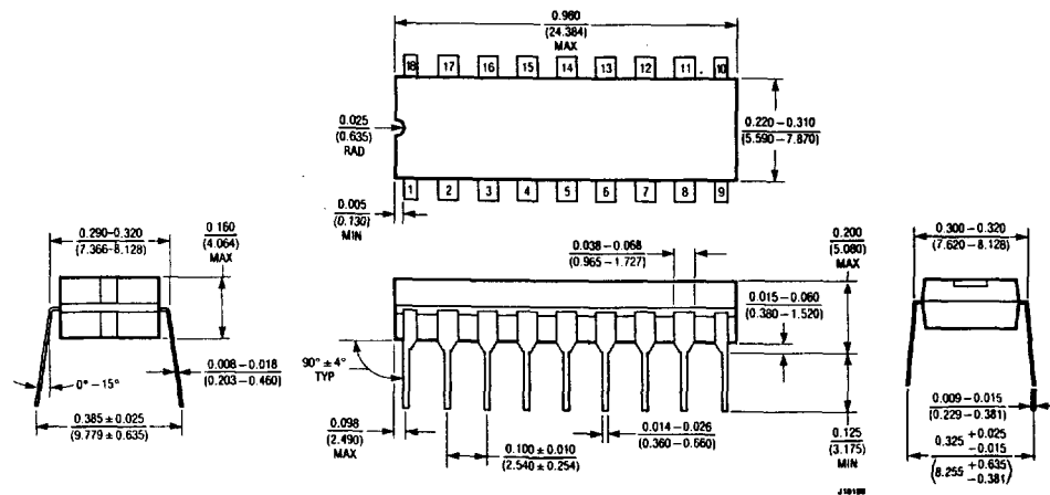
J Package 18-Lead Ceramic DIP
