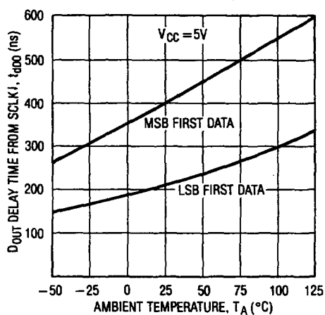
D_{\text{OUT}} Delay Time vs Temperature
