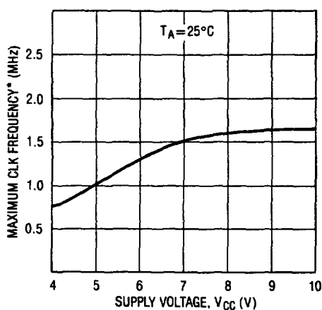
Maximum Clock Rate vs V_{\text{CC}} Supply Voltage
