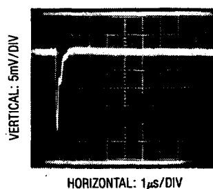
Figure 9. Adequate Settling of Op Amp Driving Analog Input
