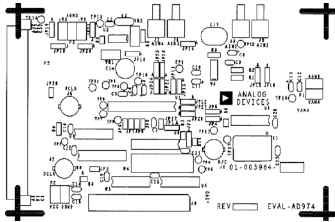
Figure 3. Component Side Silkscreen (Not to Scale)
