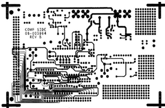
Figure 4. Component Side (Not to Scale)
