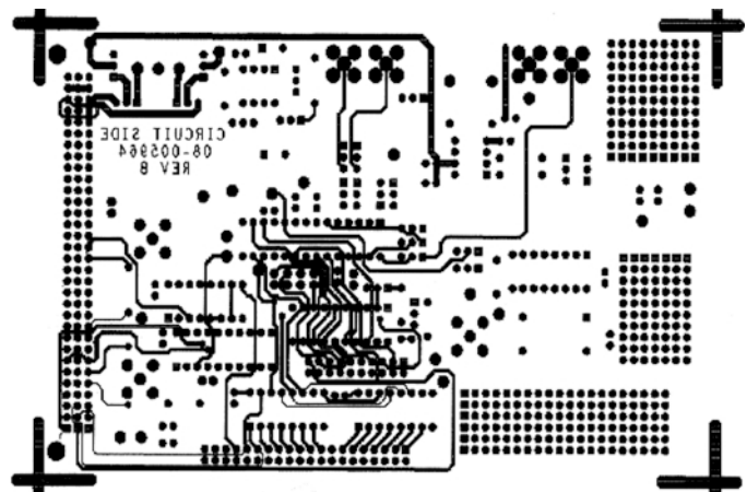
Figure 7. Circuit Side (Not to Scale)
