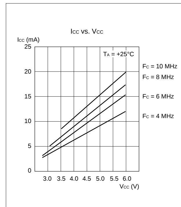
(8) Operating Supply Current vs. V_{CC}
