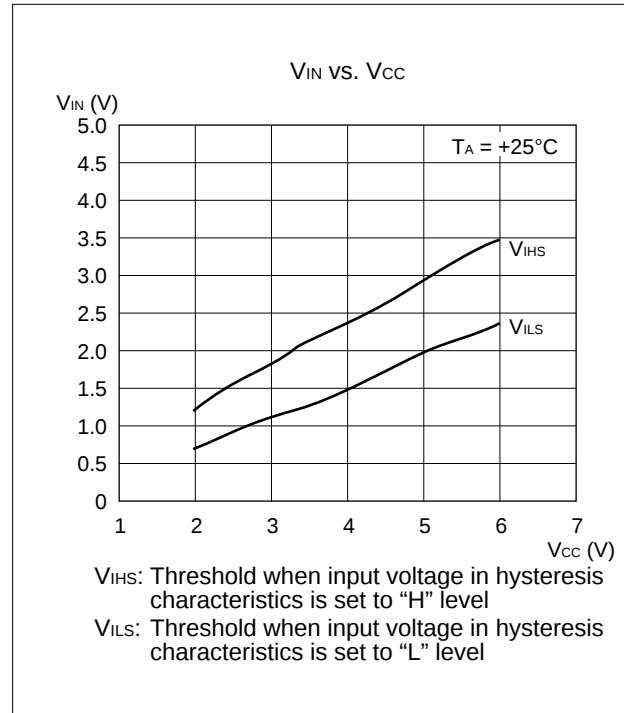
(6) "H" Level Input Voltage/"L" level Input Voltage (Hysteresis Input)
