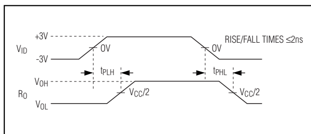
Figure 2. Propagation Delay
