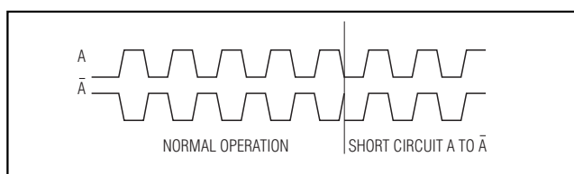
Figure 8. Short-Circuit Detection
