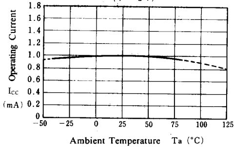
Operating Current vs. Temperature ( V^+ = 5\text{ V} )
