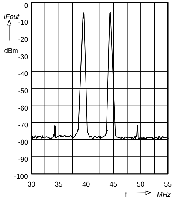
Third Order IMD
