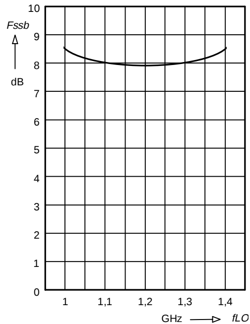
SSB Noise Figure F_{ssb} = f(fLO)
