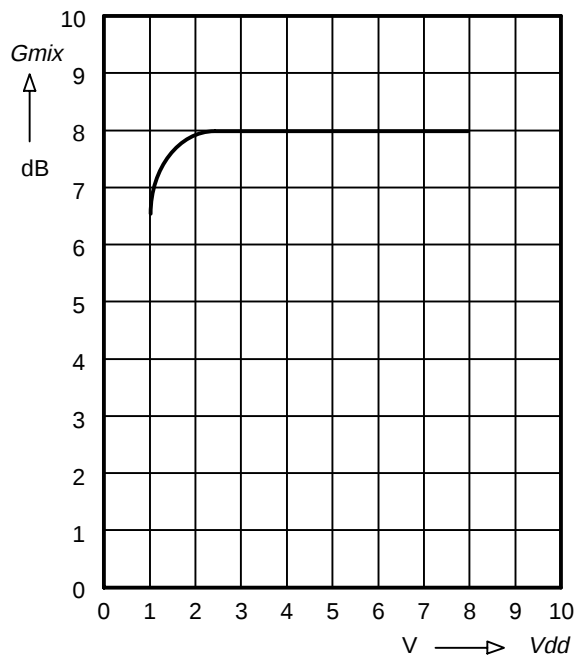
Conversion Gain G_{mix} = f(V_{dd})
