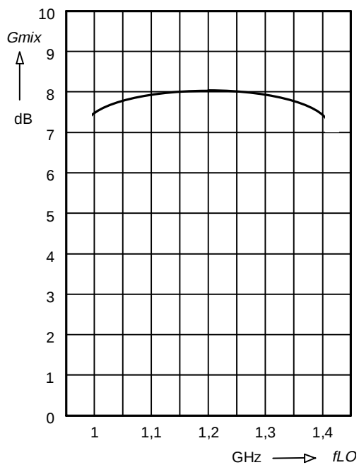
Conversion Gain G_{mix} = f(fLO)
