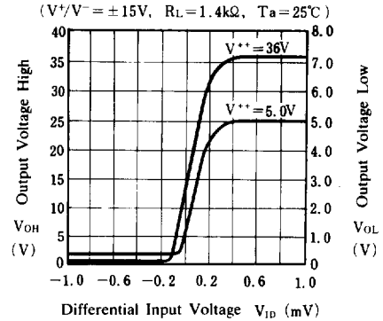
Transfer Function
