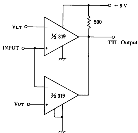
Window Detector
