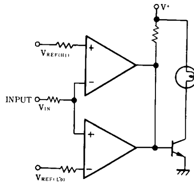
Limit Comparator
