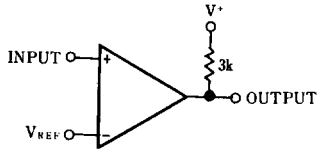
Basic Comparator
