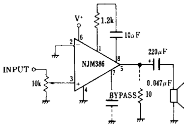
Amplifier 2
