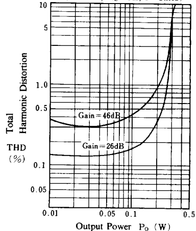
Total Harmonic Distortion vs. Output Power
