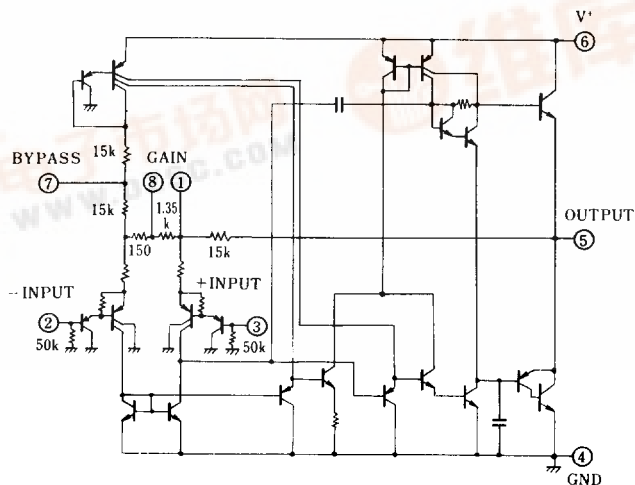
NJM386L
