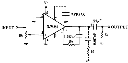
Amplifier 2
