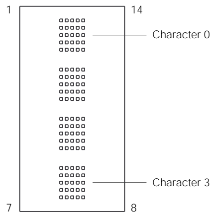
Figure 3. Top view
