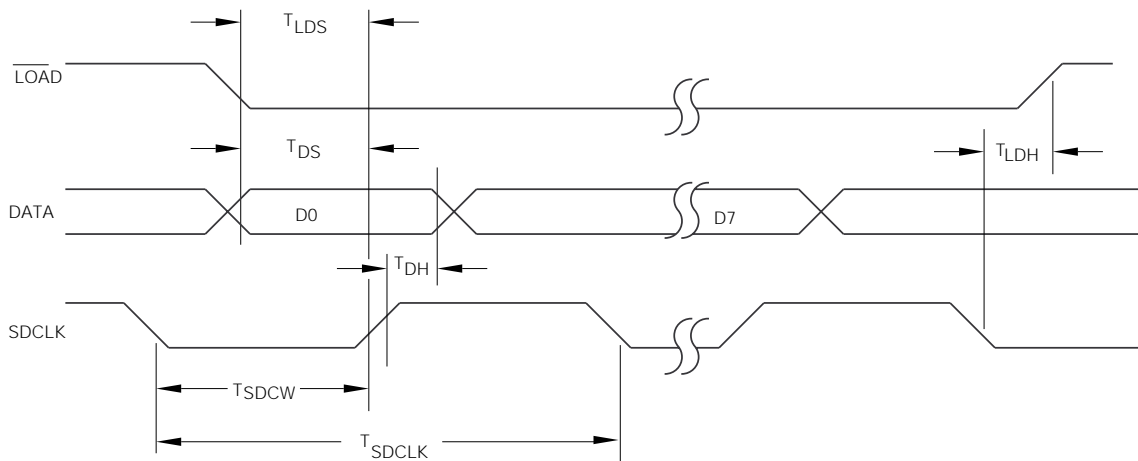
Figure 1. Timing diagram—data write cycle
