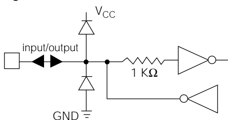
Figure 5. lock I/O
