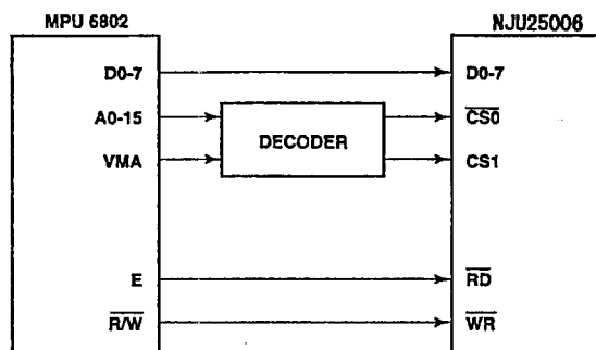
Figure 19 68K Interface
