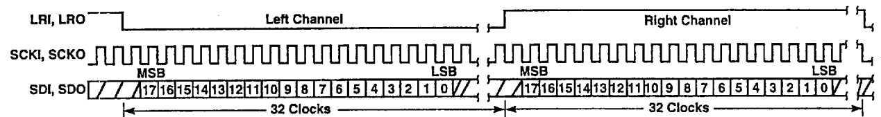
Figure 9 I^2S Data Format, ADSCK = 64 F_s , 18-bit Data
