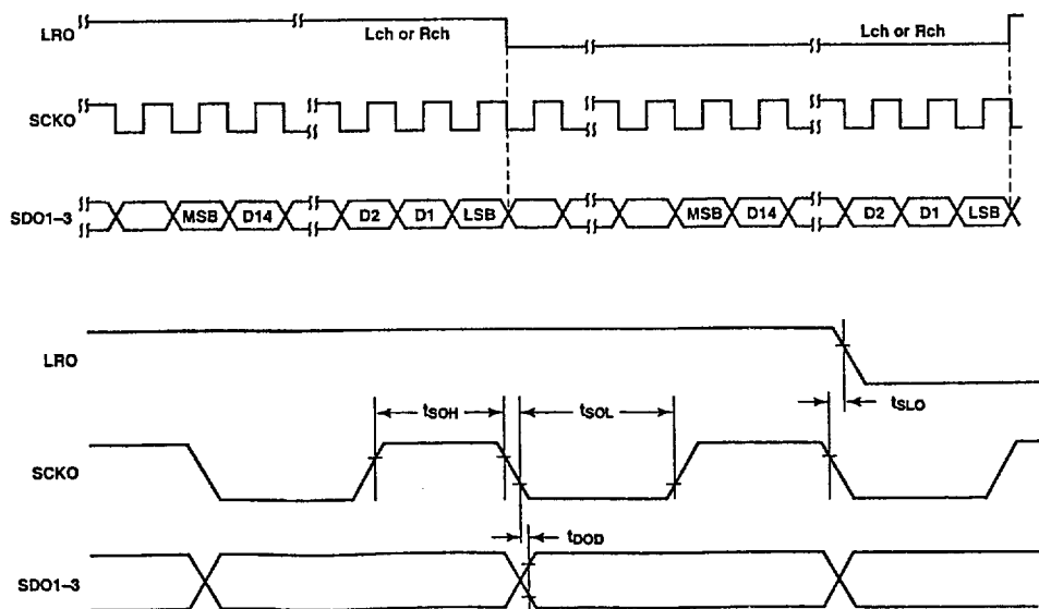
Figure 6 Serial Data Output Timing
