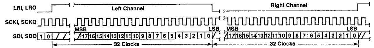
Figure 8 Right-Justified Data Format, ADSCK = 64 F_s , 18-bit Data
