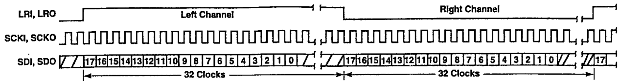
Figure 7 Left-Justified Data Format, ADSCK = 64 F_s , 18-bit Data
