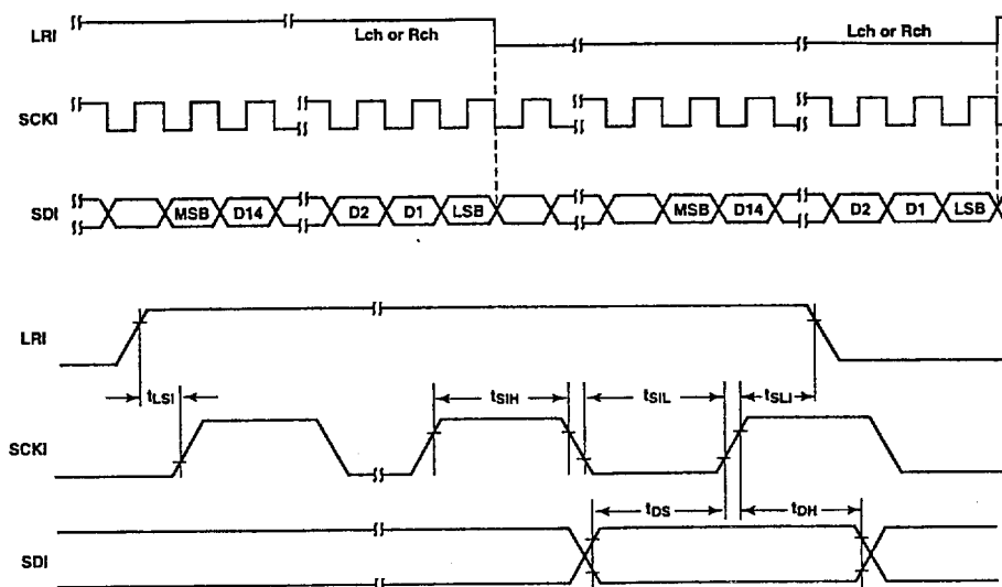
Figure 5 Serial Data Input Timing
