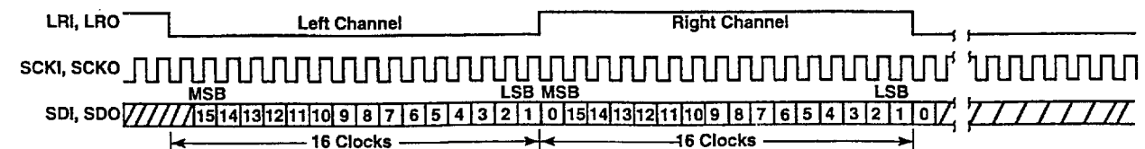
Figure 11 I^2S Data Formats, ADSCK = 32 F_s , 16-bit Data
