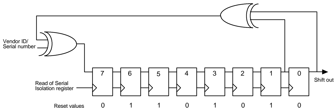
Figure 3. Checksum LFSR
