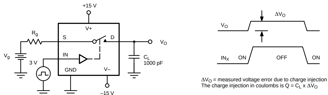
FIGURE 5. Charge Injection
