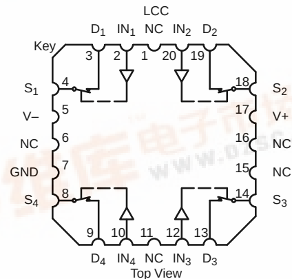
DG201A_MIL
