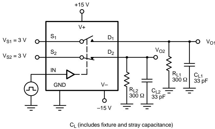
FIGURE 3. Break-Before-Make SPDT (DG305A, DG307A)
