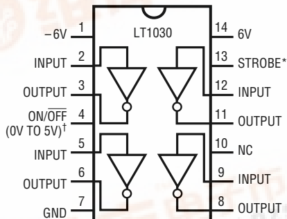
RS232 Line Driver
