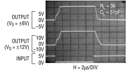
Output Waveforms
