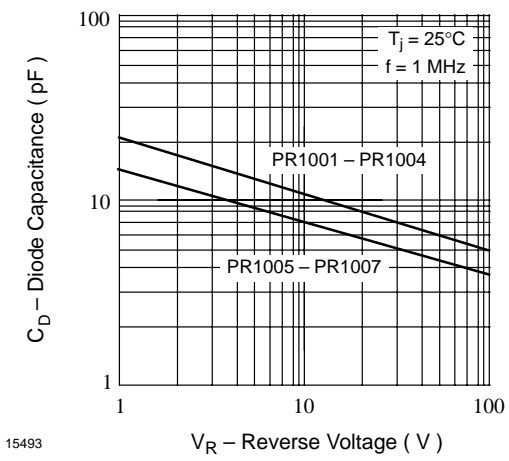
Figure 4. Typ. Diode Capacitance vs. Reverse Voltage
