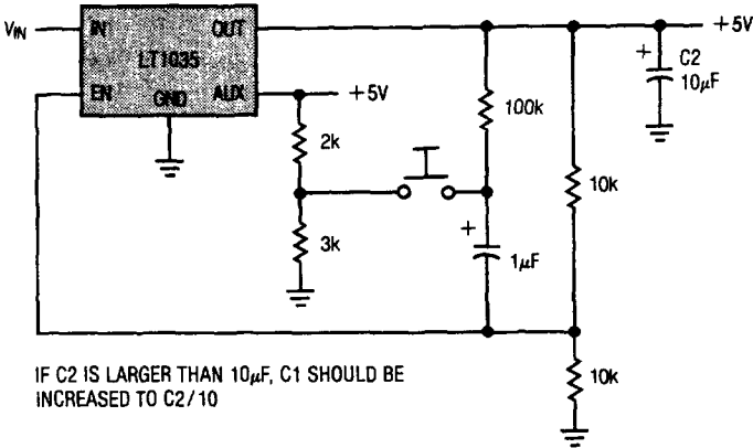
Push-On, Push-Off
