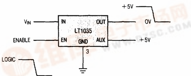
Functional Diagram
