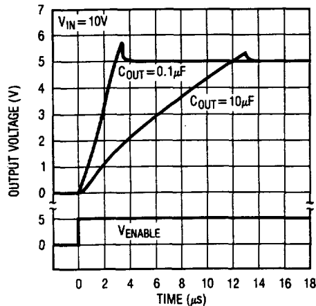
Output Switching Characteristics
