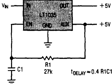
Delayed Power-Up
