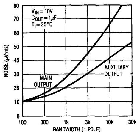
Output Noise
