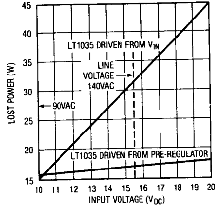
Regulator Losses at I_{OUT} = 3A
