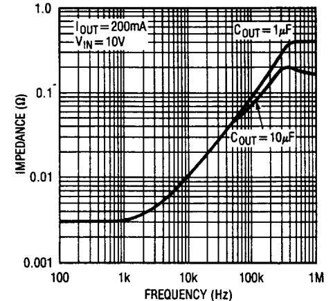
Output Impedance
