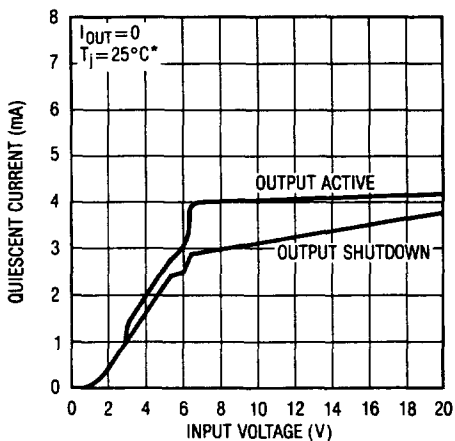
Quiescent Current
