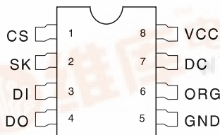
8-Pin SOIC
