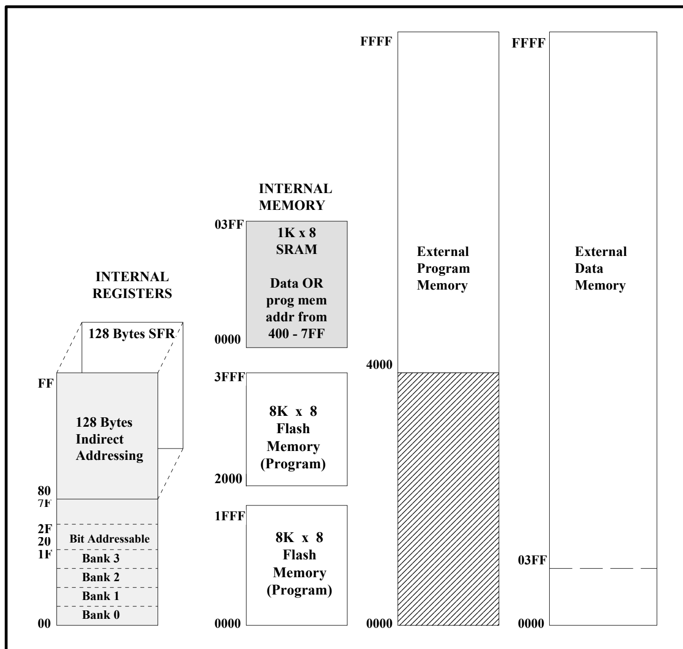
Figure 6. Memory Map (as shown for the DS89C430)
