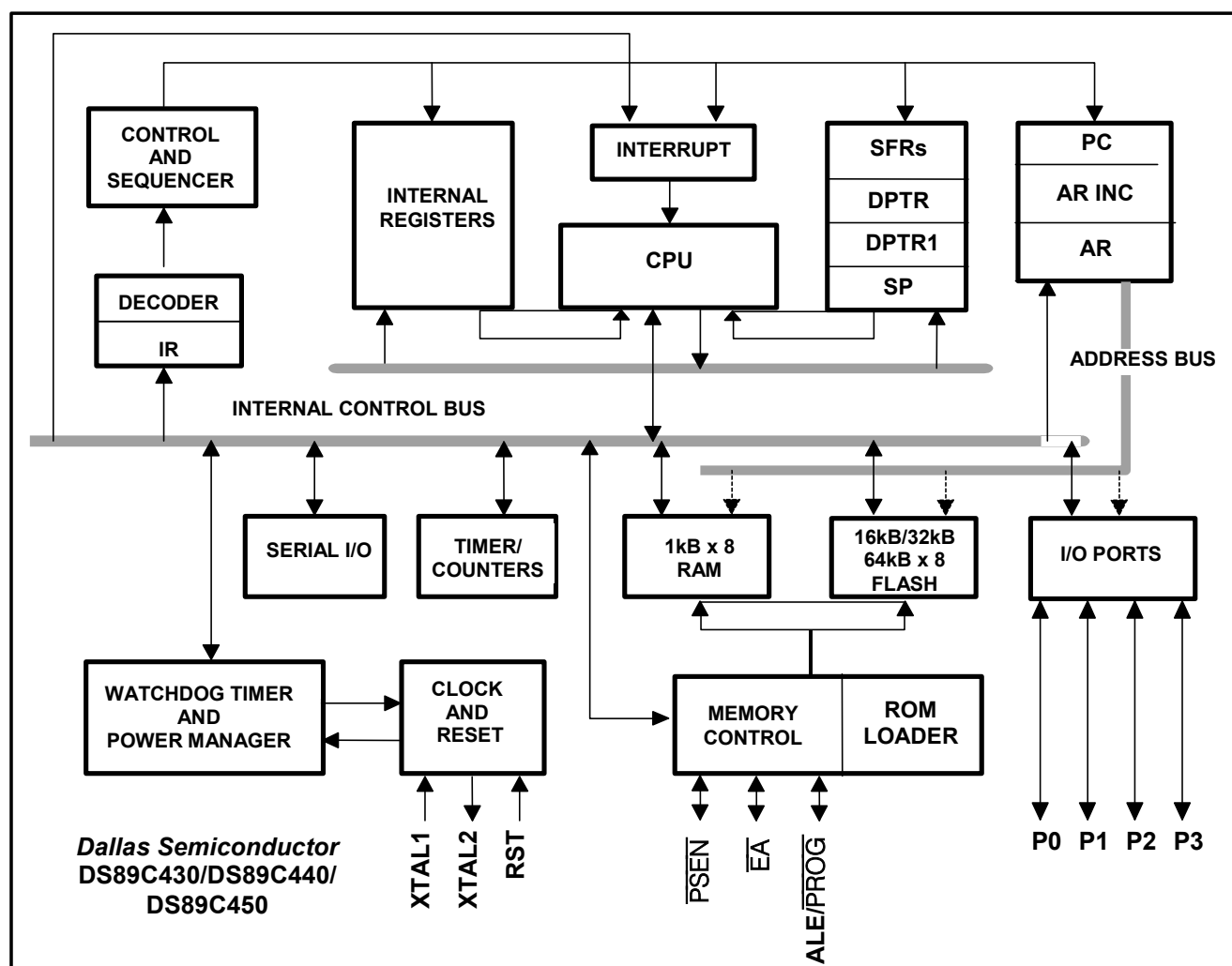
Figure 5. Functional Diagram
