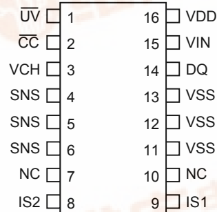
DS2770 16-Pin TSSOP
