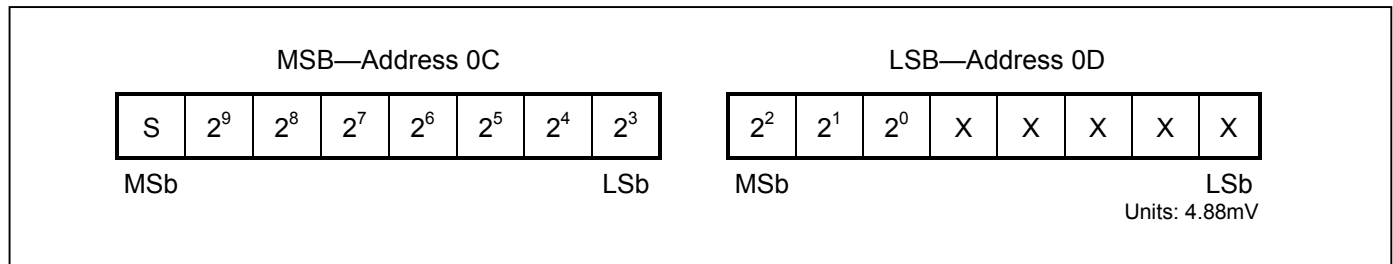
Figure 7. Voltage Register Format
