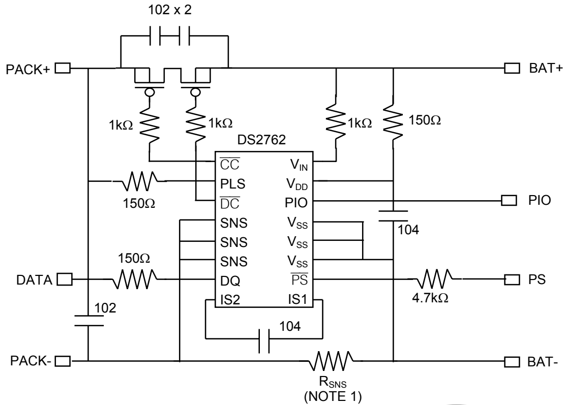
Figure 2. Application Example
