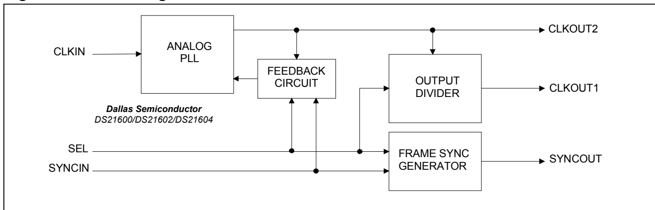
Figure 1-1. Block Diagram
