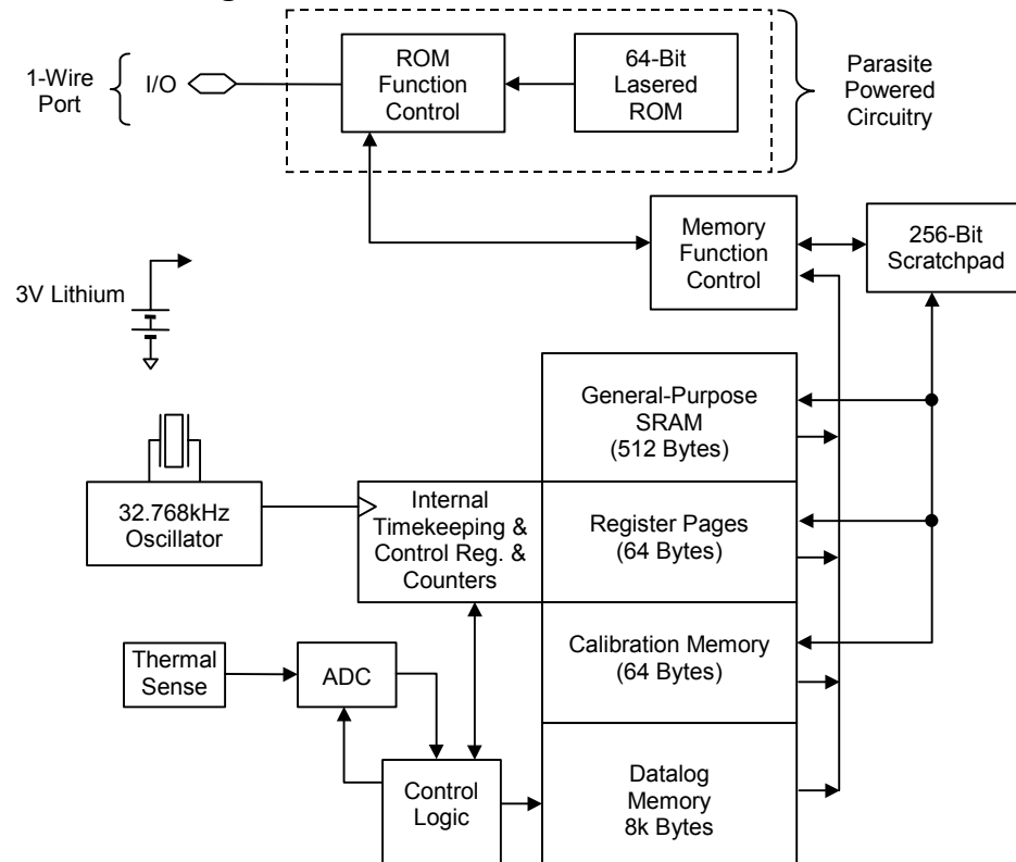
Figure 1. DS1922L/T Block Diagram
