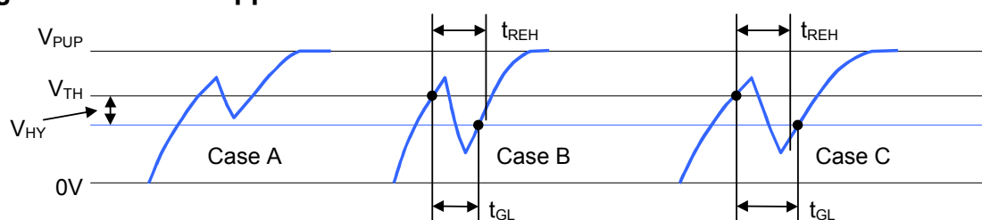
Figure 14. Noise Suppression Scheme
