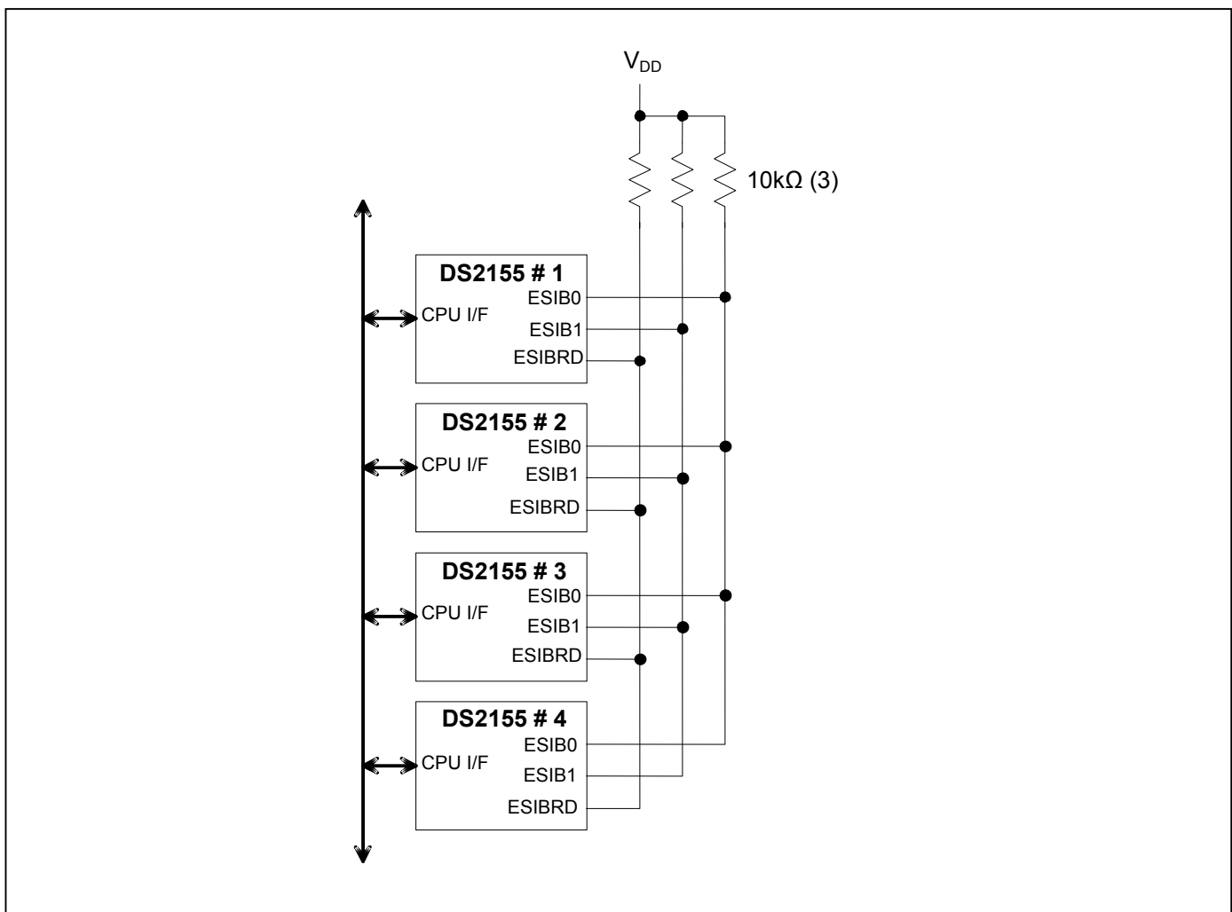
Figure 29-1. ESIB Group of Four DS2155s
