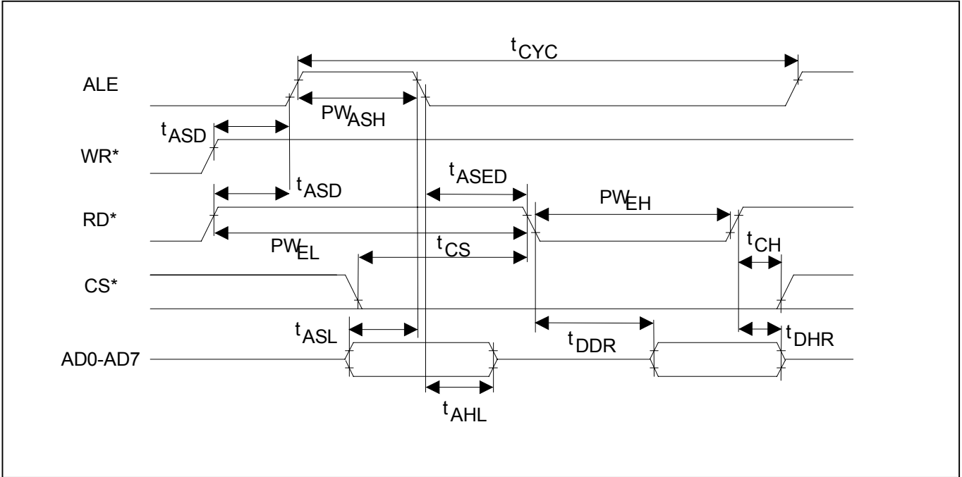
Figure 37-1. Intel Multiplexed Bus Read Timing (BTS = 0/MUX = 1)
