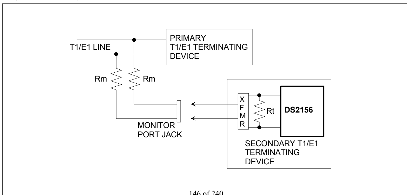
Figure 24-1. Typical Monitor Application
