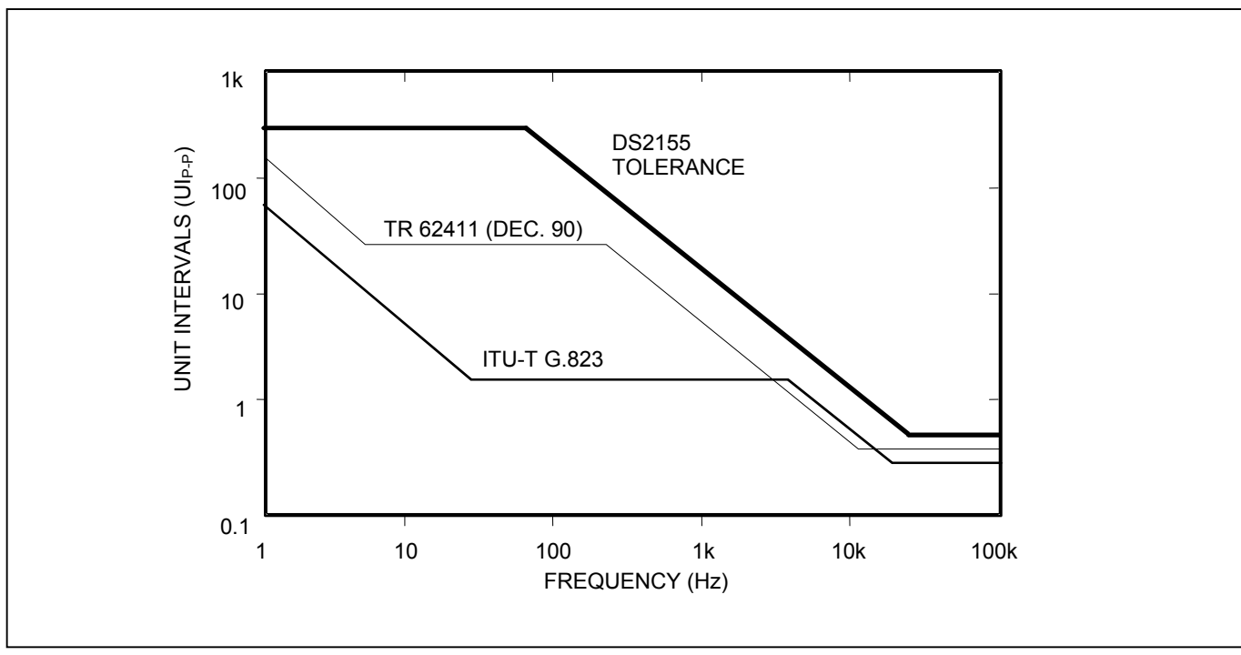
Figure 24-7. Jitter Tolerance
