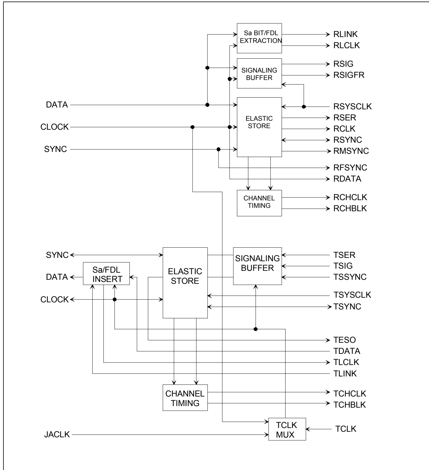
Figure 3-4. Backplane Interface
