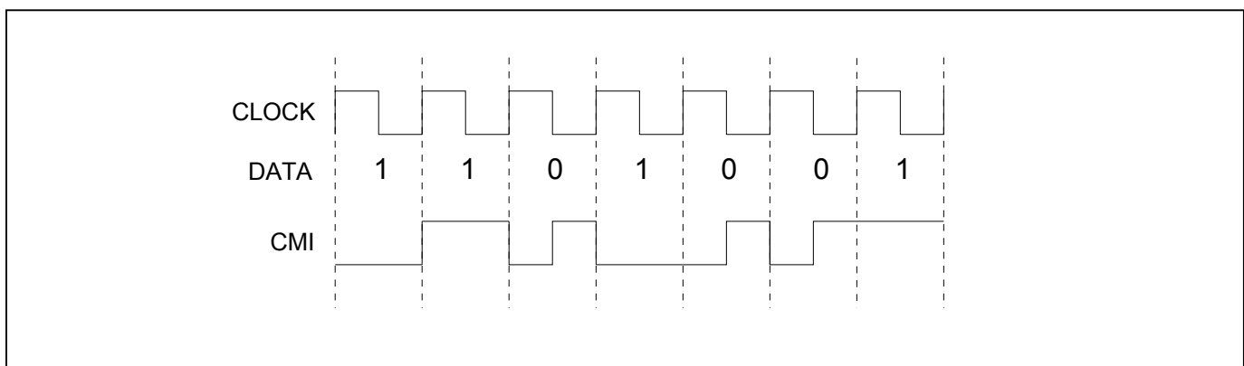
Figure 24-2. CMI Coding
