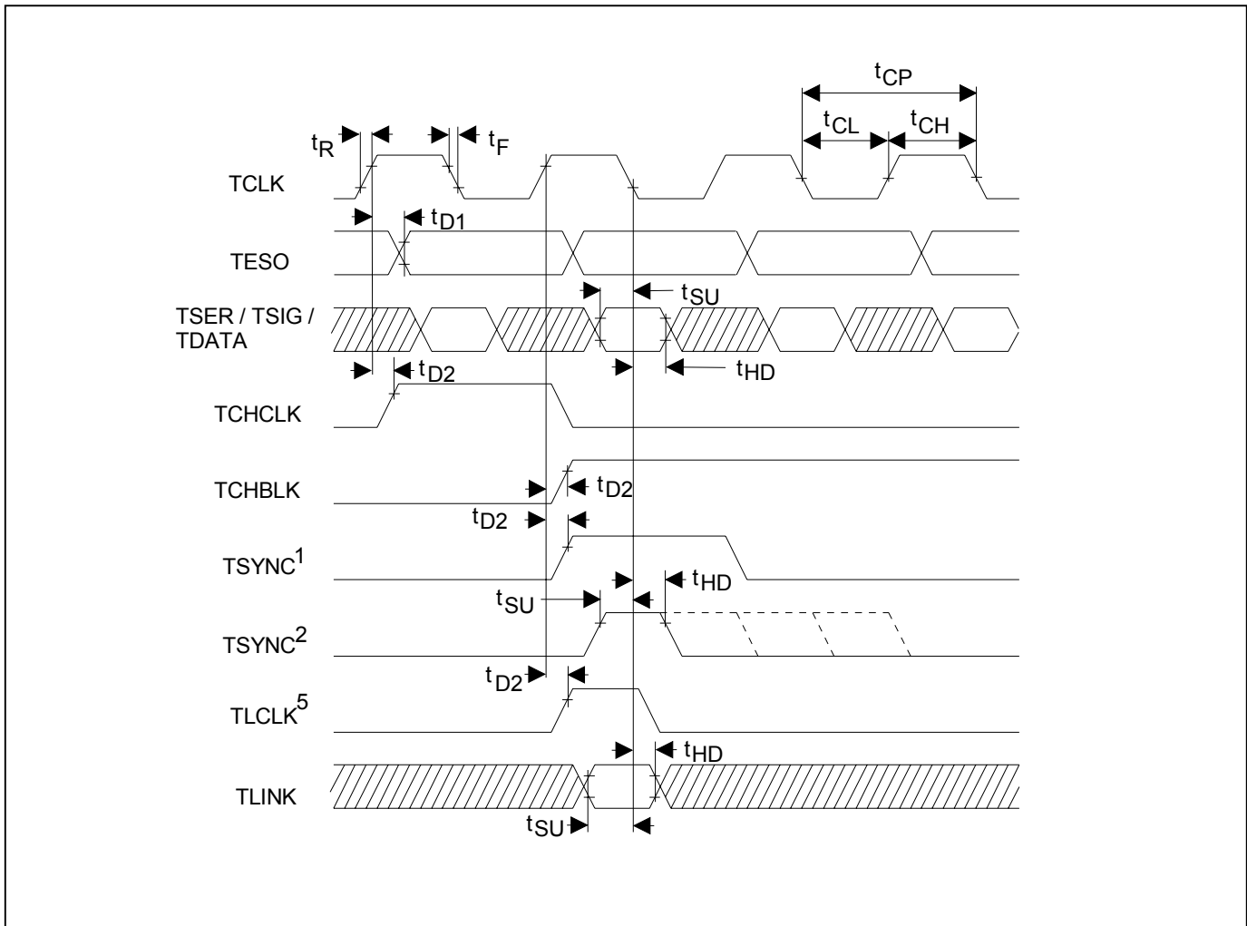
Figure 37-12. Transmit-Side Timing
