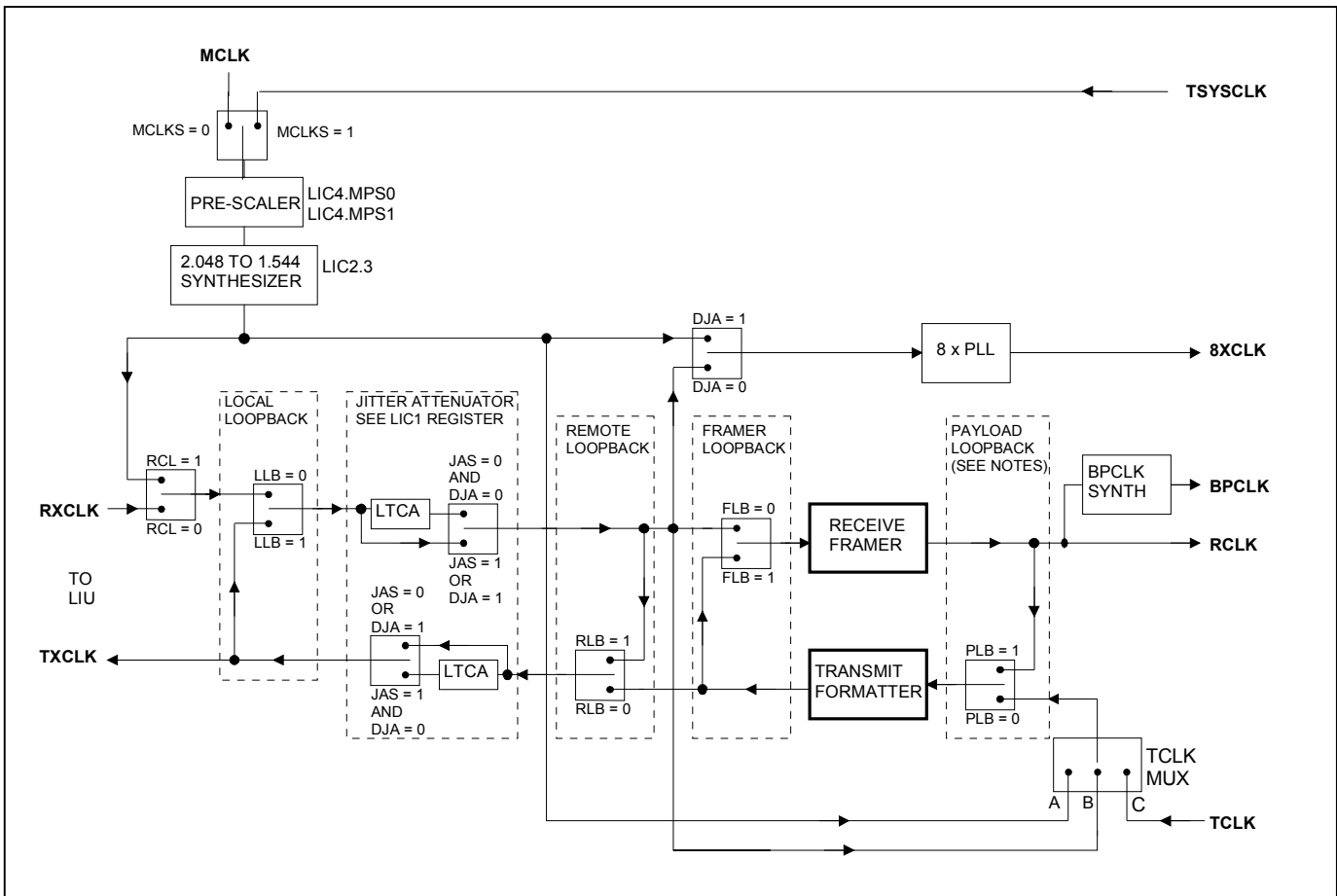
Figure 8-1. Clock Map
