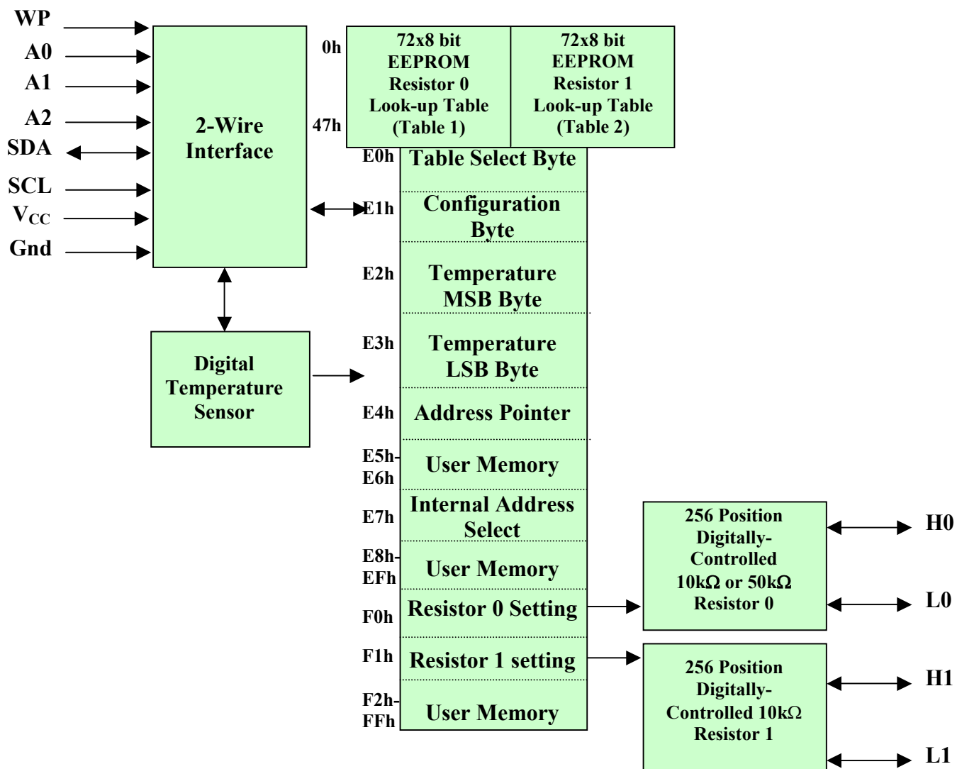
DS1847 BLOCK DIAGRAM Figure 1
