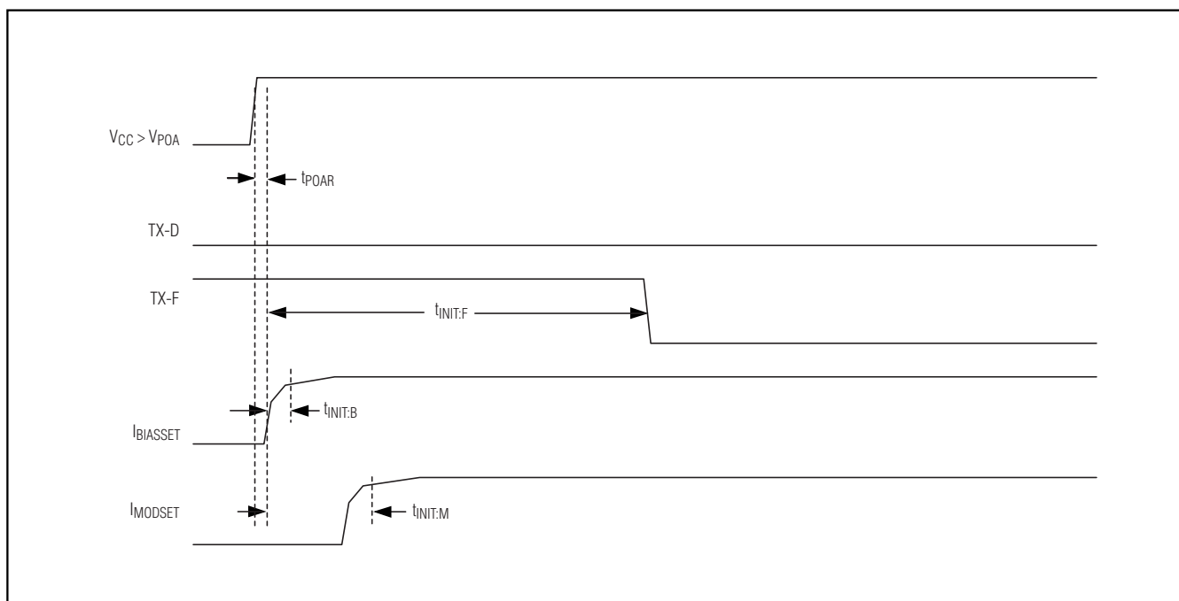
Figure 1. Power-Up Timing with TX-D Not Asserted (Including Hotplug)
