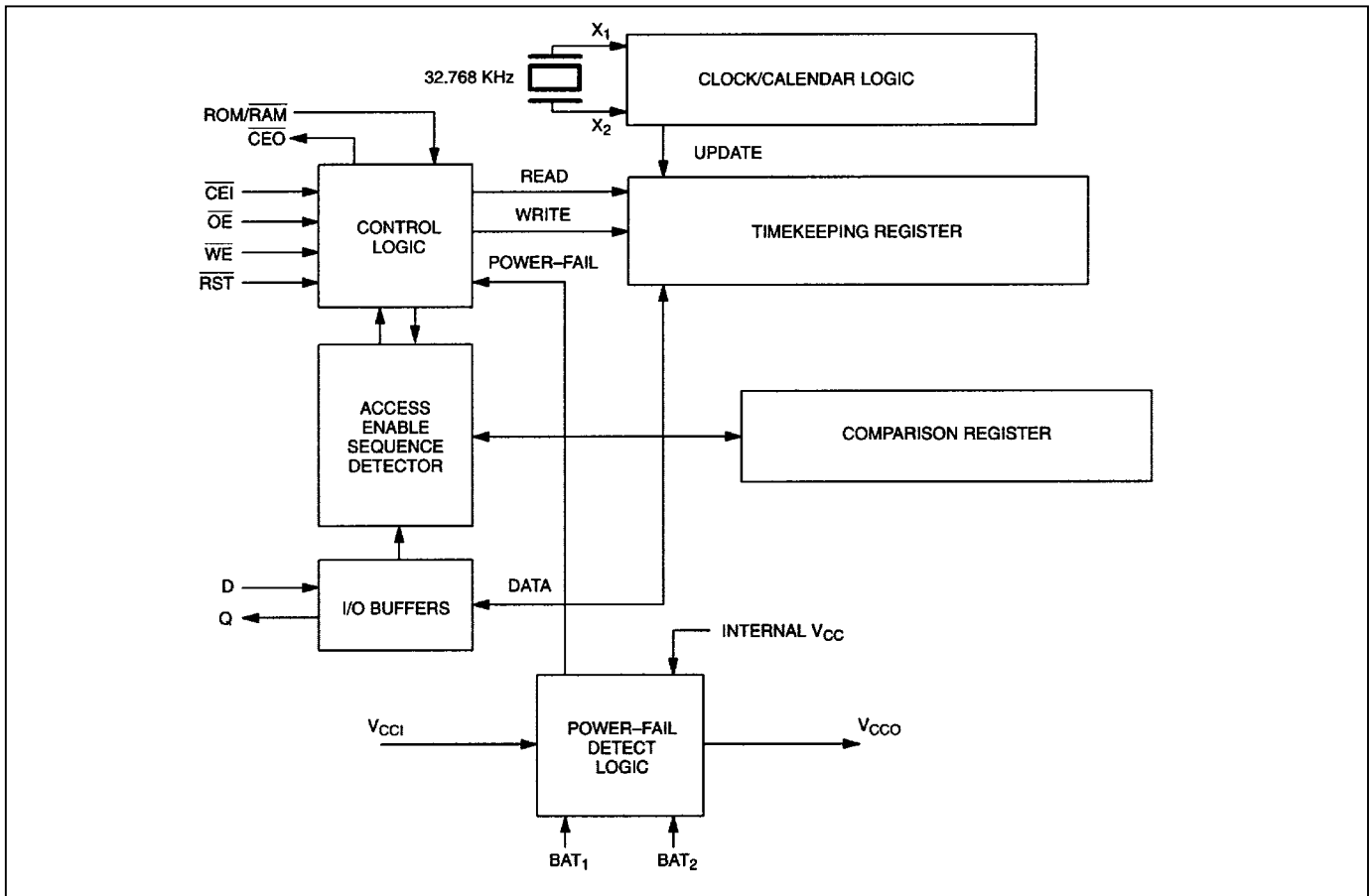
Figure 1. Block Diagram
