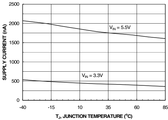
Figure 3. I SHUTDOWN Current vs. Temperature
