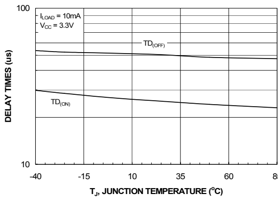
Figure 11. T_{ON}/T_{Off} vs. Temperature
