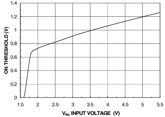
Figure 10. On Threshold vs. V_{IN}
