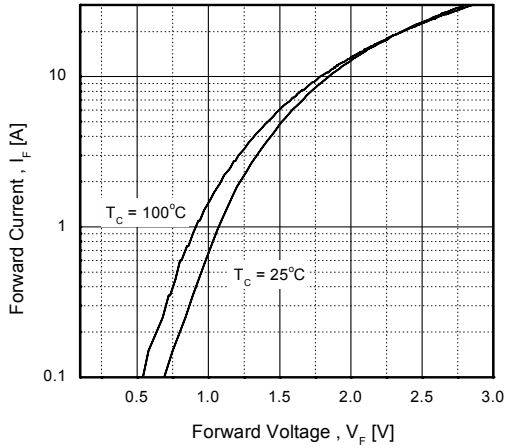
Figure 17. Forward Voltage Characteristics
