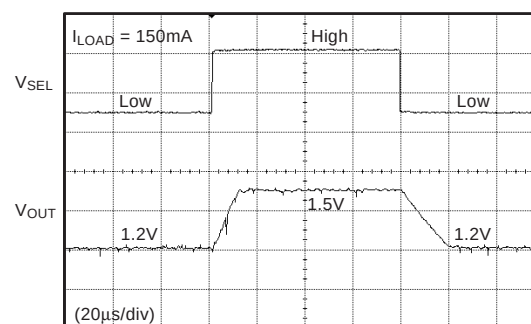
Dynamic V_{OUT} Change (FAN5631)
