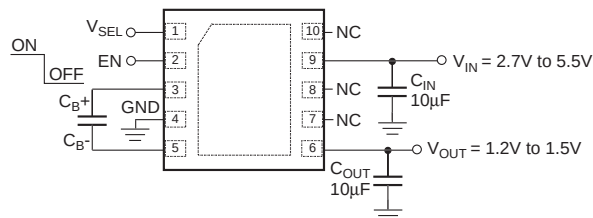
Figure 1. Typical Application
