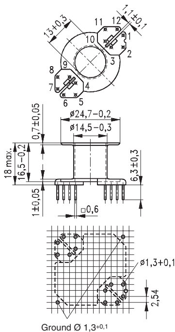
Hole arrangement View in mounting direction
