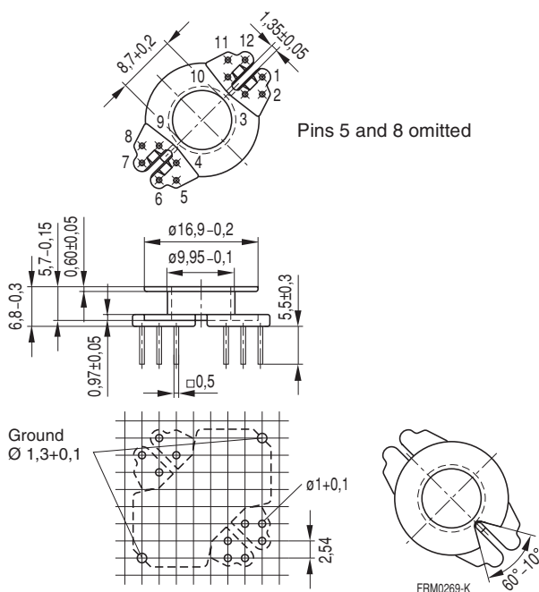
Hole arrangement View in mounting direction
