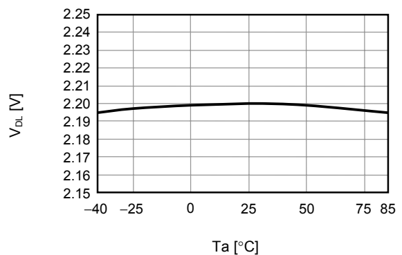
4. V_{DL} - Ta
