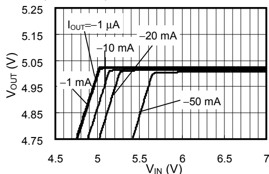
S-812C50B( T_a=25^\circ\text{C} )
