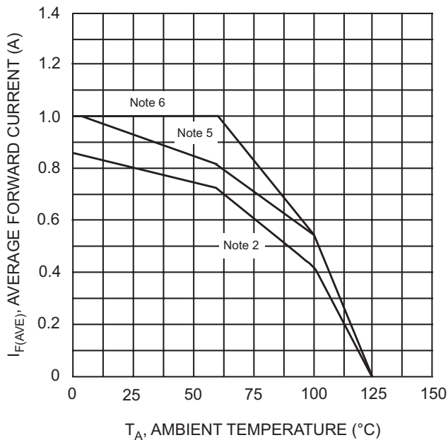
Fig. 1 Forward Current Derating
