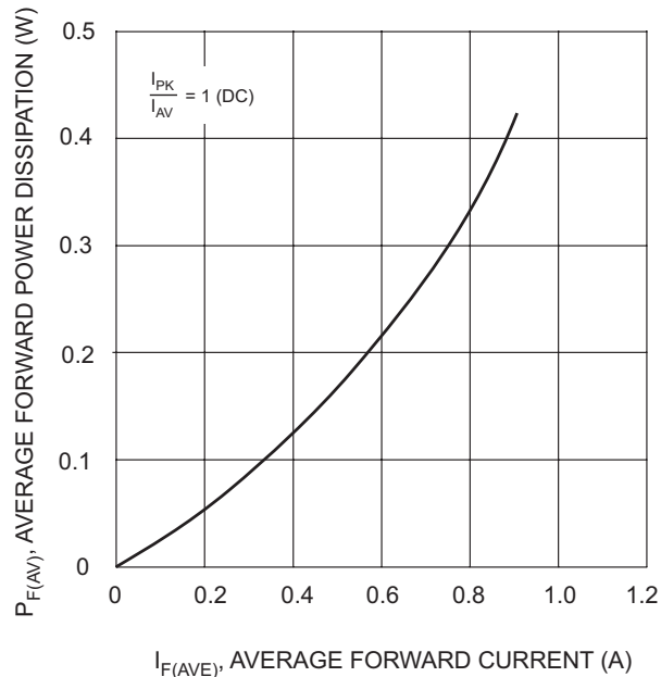
Fig. 6 Forward Power Derating
