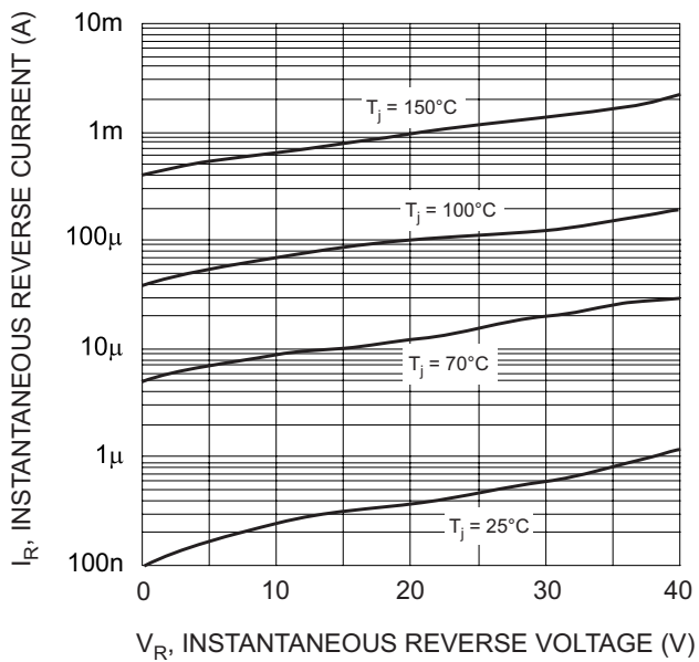
Fig. 3 Typical Reverse Current vs. Reverse Voltage
