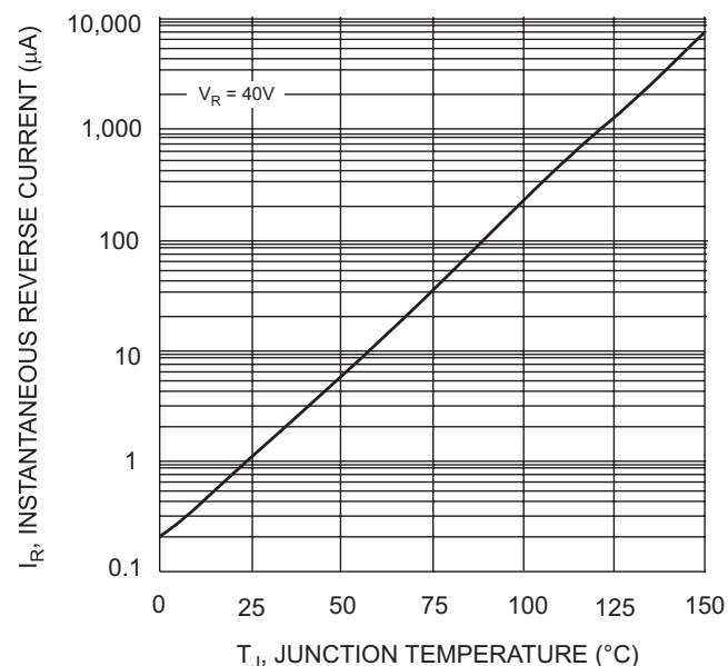
Fig. 4 Typical Reverse Current vs. Junction Temperature
