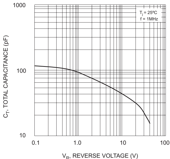
Fig. 5 Typical Total Capacitance vs. Reverse Voltage
