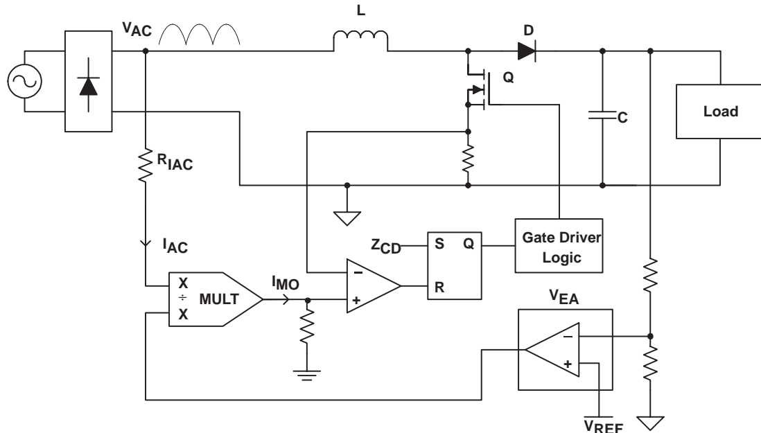
Figure 1. Basic Block Diagram of CRM Boost PFC
