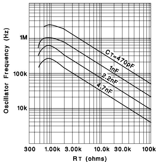
Figure 6. Oscillator
