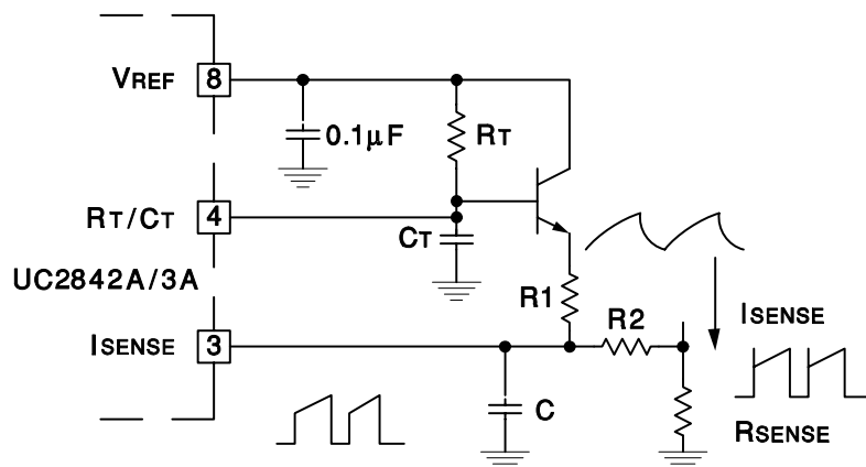
Figure 8. Slope Compression
