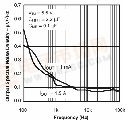
TPS79630 OUTPUT SPECTRAL NOISE DENSITY VS FREQUENCY
