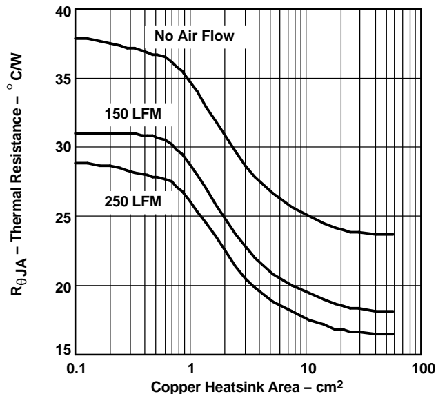
Figure 20. DDPAK Thermal Resistance vs Copper Heatsink Area
