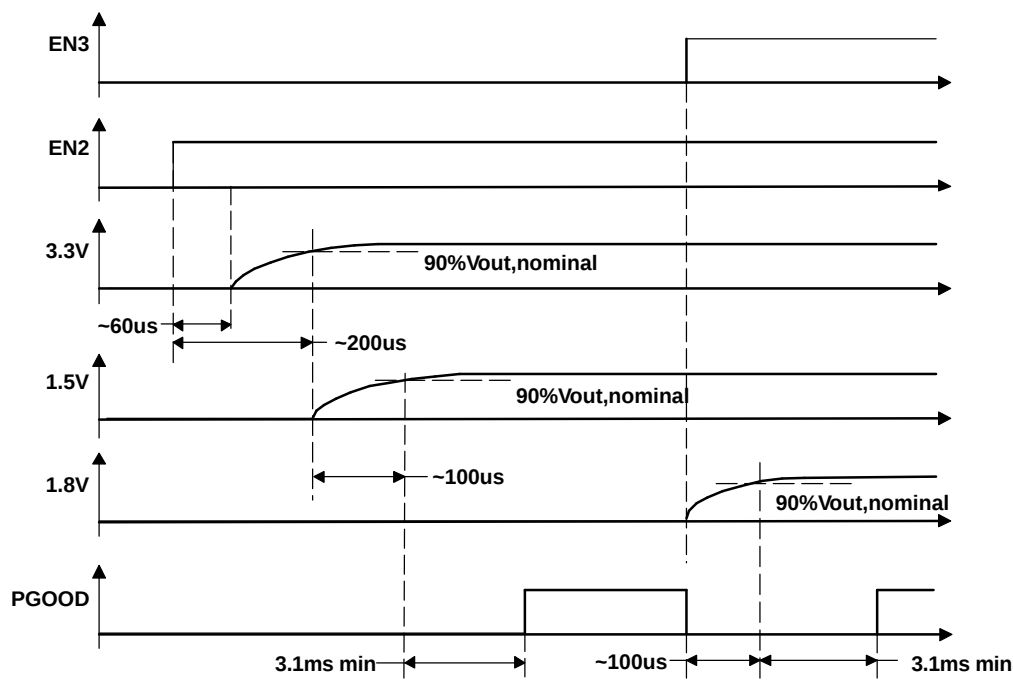
Figure 16. Timing Diagram
