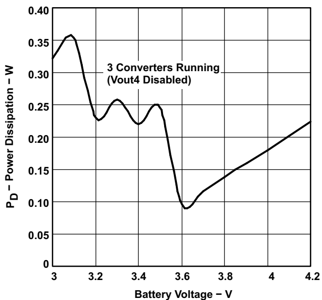
Figure 19. Power Dissipation vs Battery Voltage
