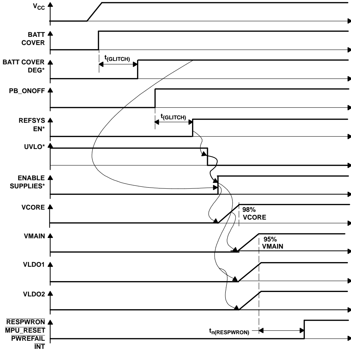
Figure 32. State 1 to State 2 Transition (PS_SEQ = 0, V CC > V UVLO + HYST)
