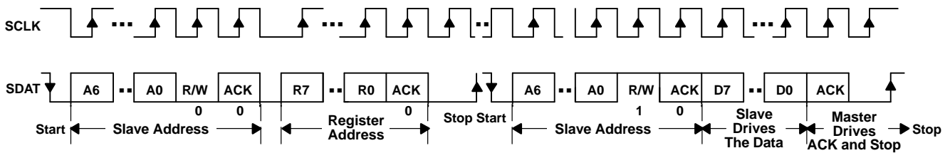
Figure 43. Serial Interface READ From TPS65014: Protocol B
