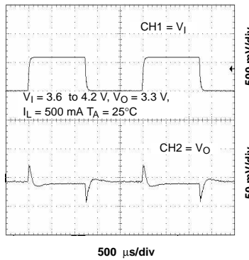
LINE TRANSIENT RESPONSE (MAIN)
