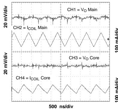
OUTPUT RIPPLE (PWM = 1)
