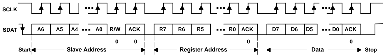
Figure 41. Serial Interface WRITE to TPS65013 Device
