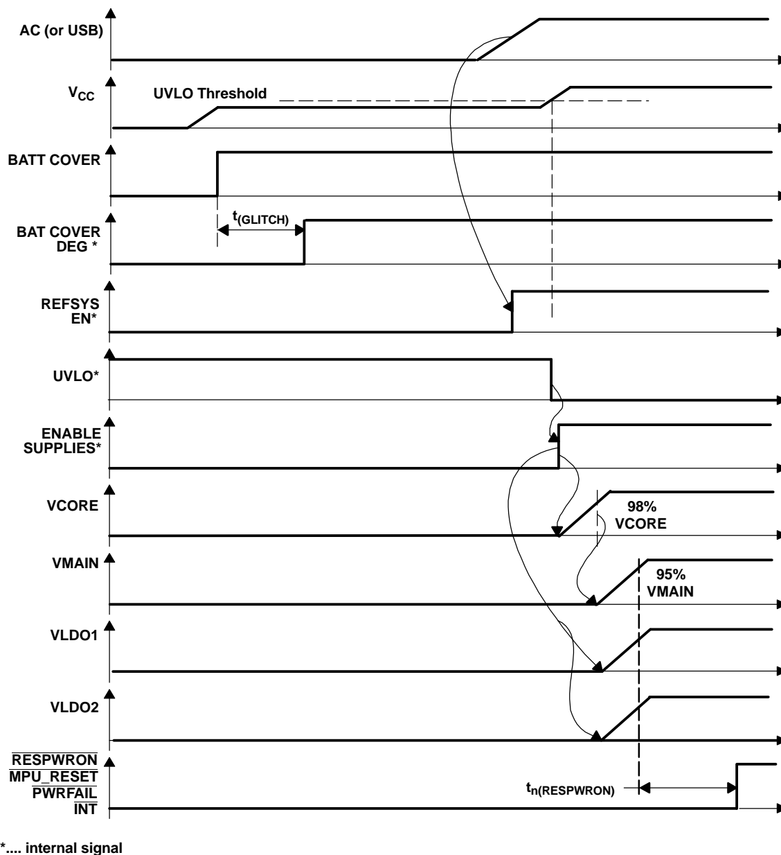
Figure 33. State1-State4-State 2 Transition (Power up behavior when Charge Voltage is Applied)
