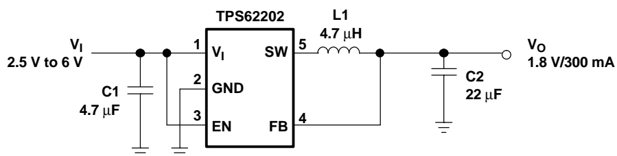
Figure 19. 1.8 V Fixed Output Voltage version Using 4.7 \mu\text{H} Inductor
